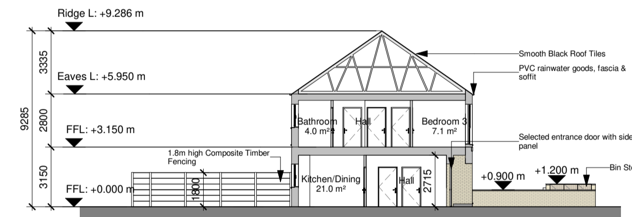
8 House Block HB1 - Section 1 : 200
