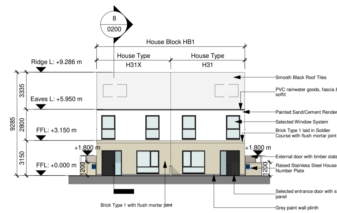
4 House Block HB1 - Front Elevation 1 : 200
