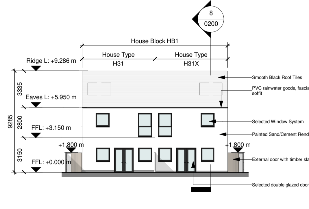
5 House Block HB1 - Rear Elevation 1 : 200
