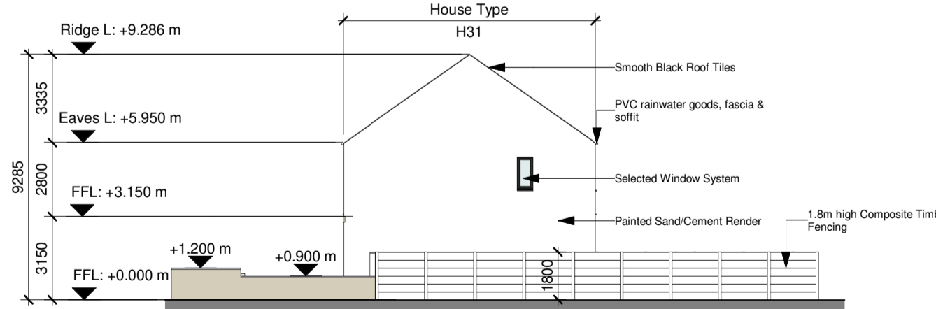
7 House Block HB1 - Side Elevation 02 1 : 200
