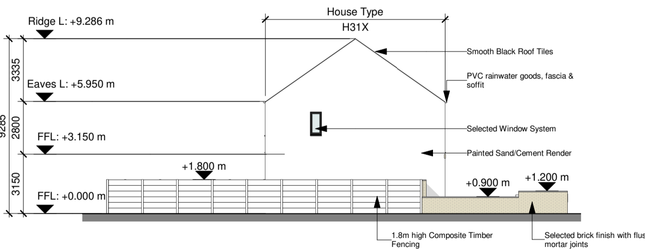
6 House Block HB1 - Side Elevation 01 1 : 200
