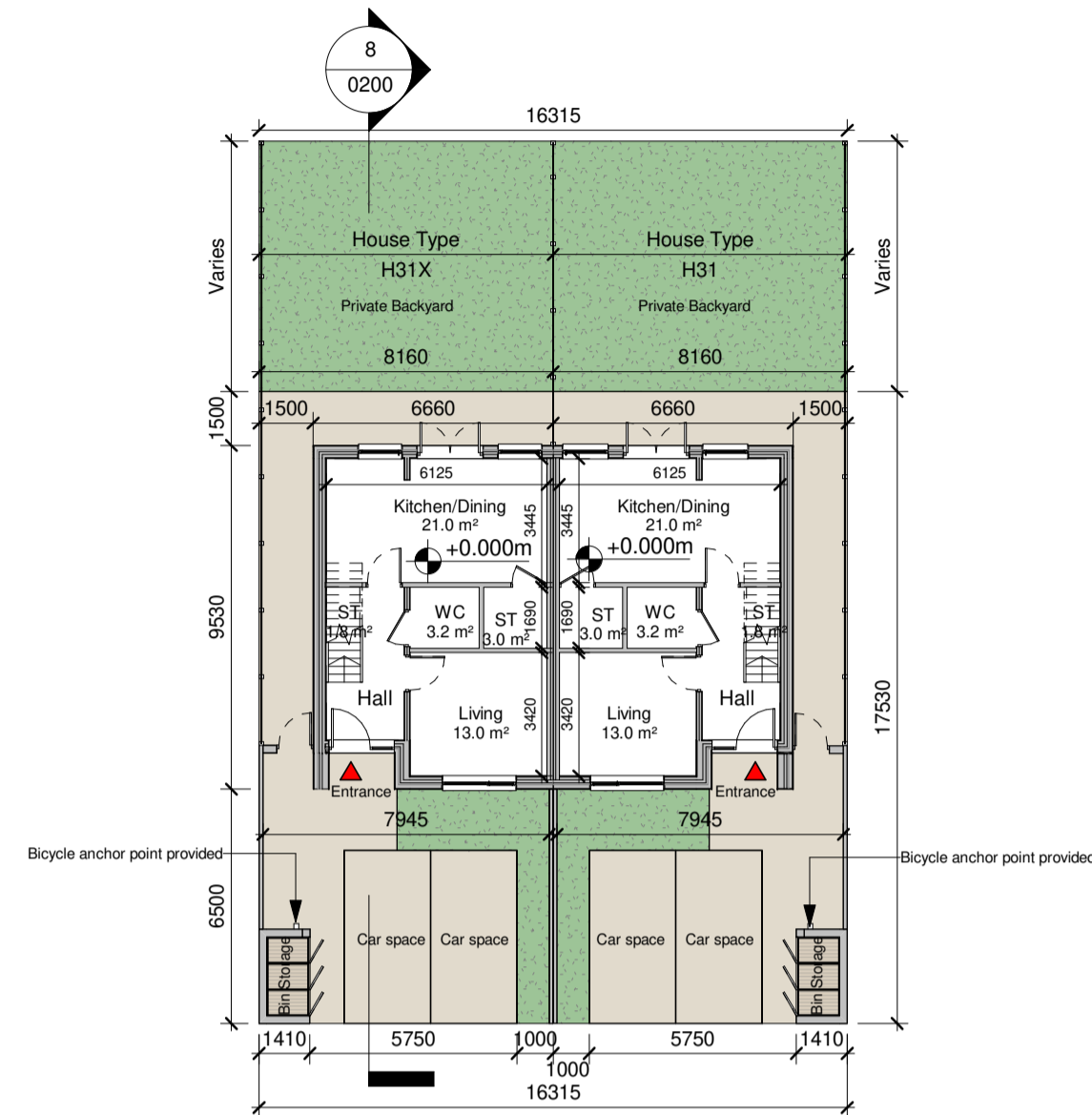
1 House Block HB1 - Ground Floor Plan 1 : 200
