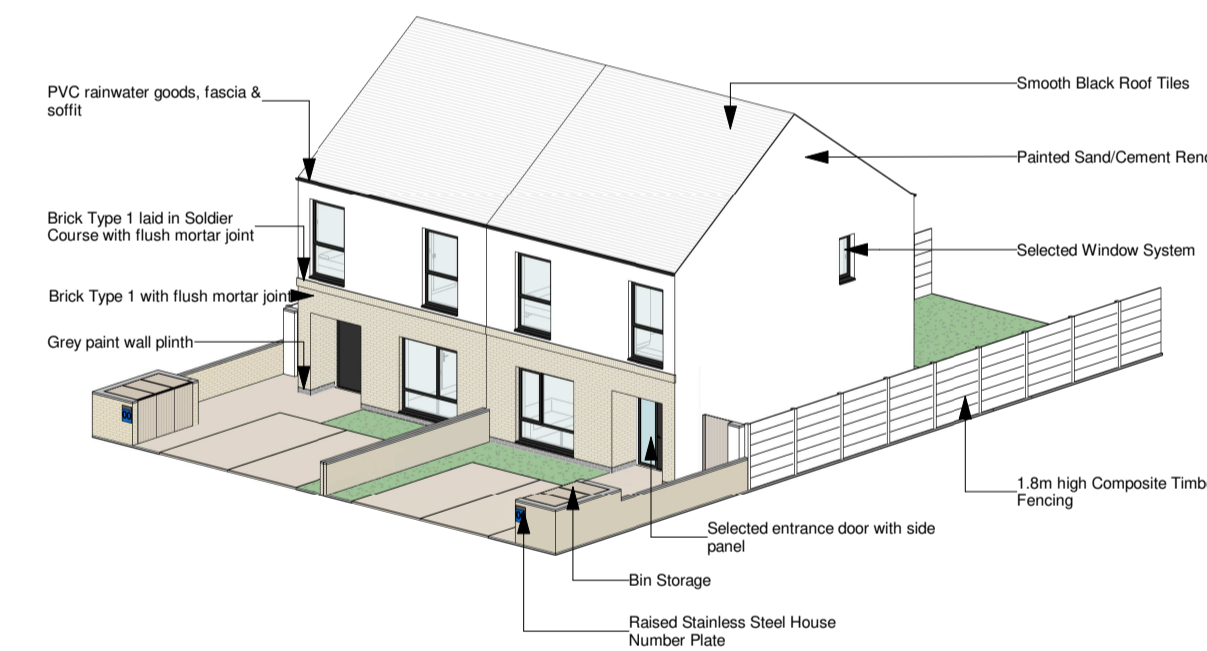
9 House Block HB1 - Axonometric View
